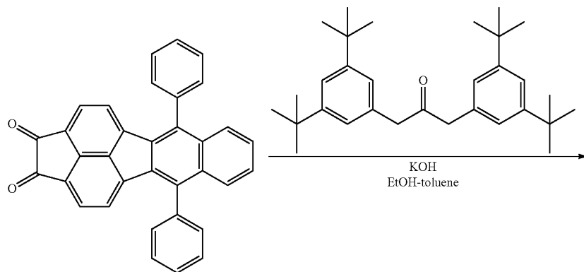
Intermediate D
