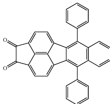
Intermediate D
