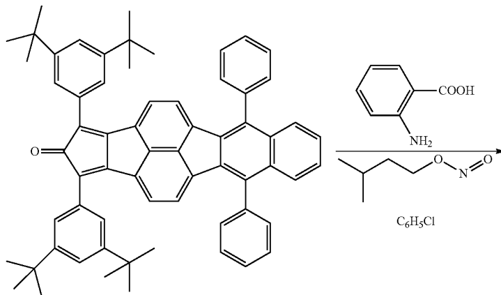
Intermediate F
