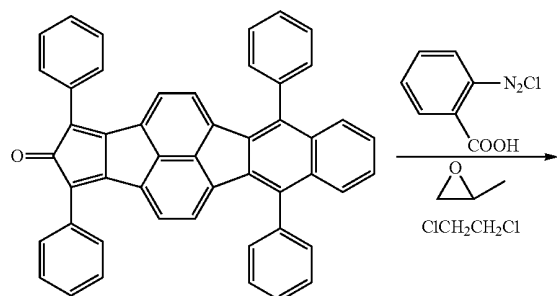
Intermediate E
