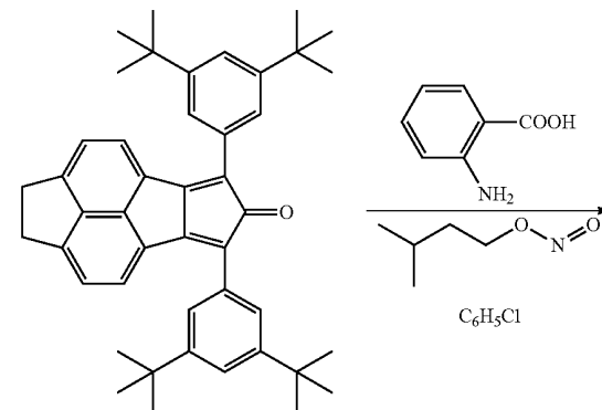
Intermediate A
