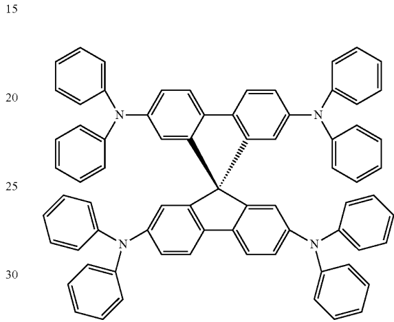
spiro-TPD
