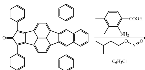
Intermediate E
