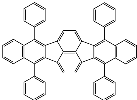
Comparative Compound 1
