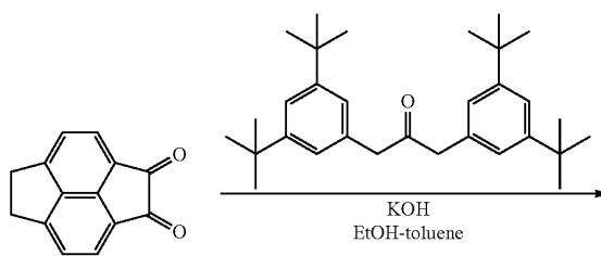
Intermediate A
