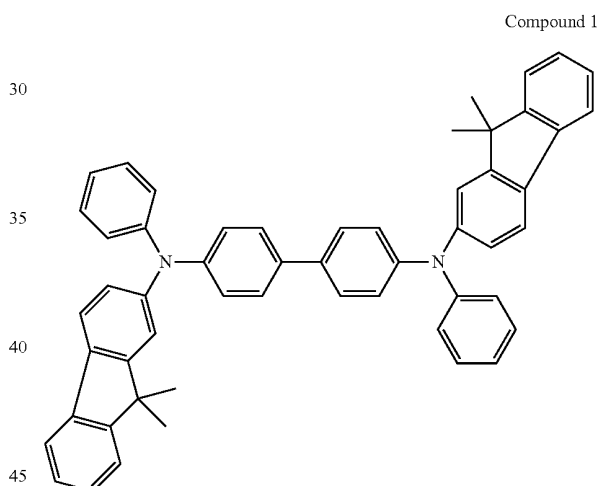
Compound 1
