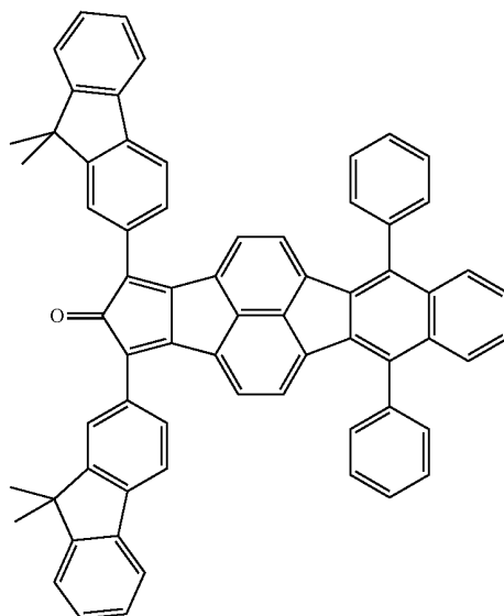
Intermediate G
