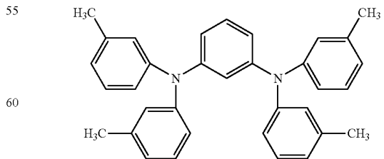
PDA
